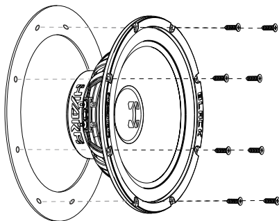
Installation of the midwoofer speaker without grill
