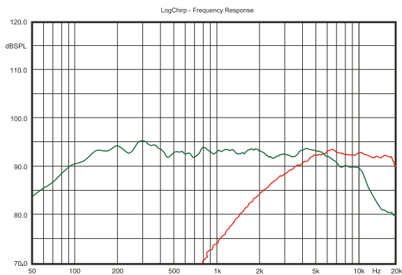
Crossover DELTA 613C
