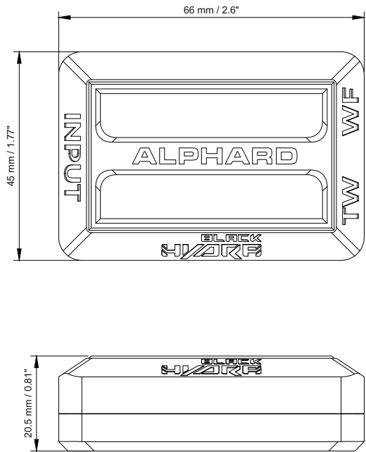
Crossover DELTA 613C
