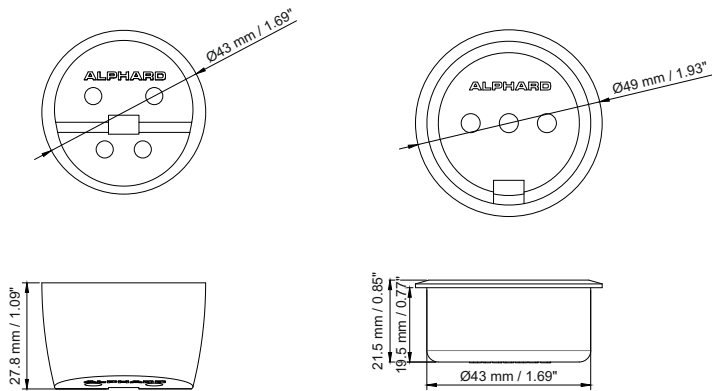
Mounting cups
