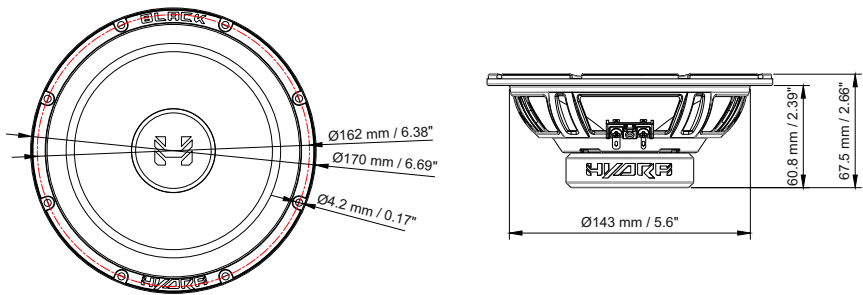
Midwoofer speaker DELTA 613C
