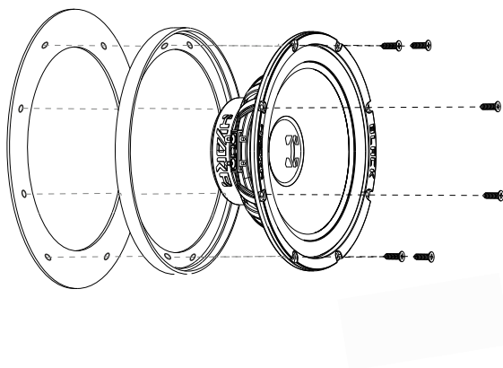
Installation of the midwoofer speaker with use of spacers
