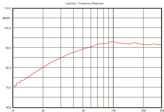
Crossover DELTA 613C
